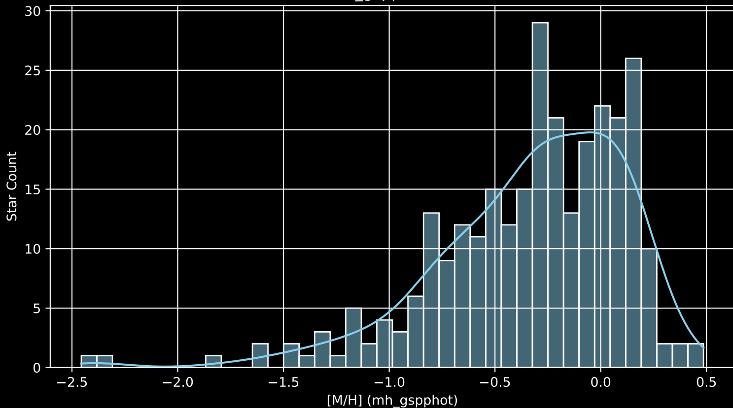
APOGEE DR17 Field: [K2_C11_001+07_btx [M/H] (mh_gspphot) (n= 286)
