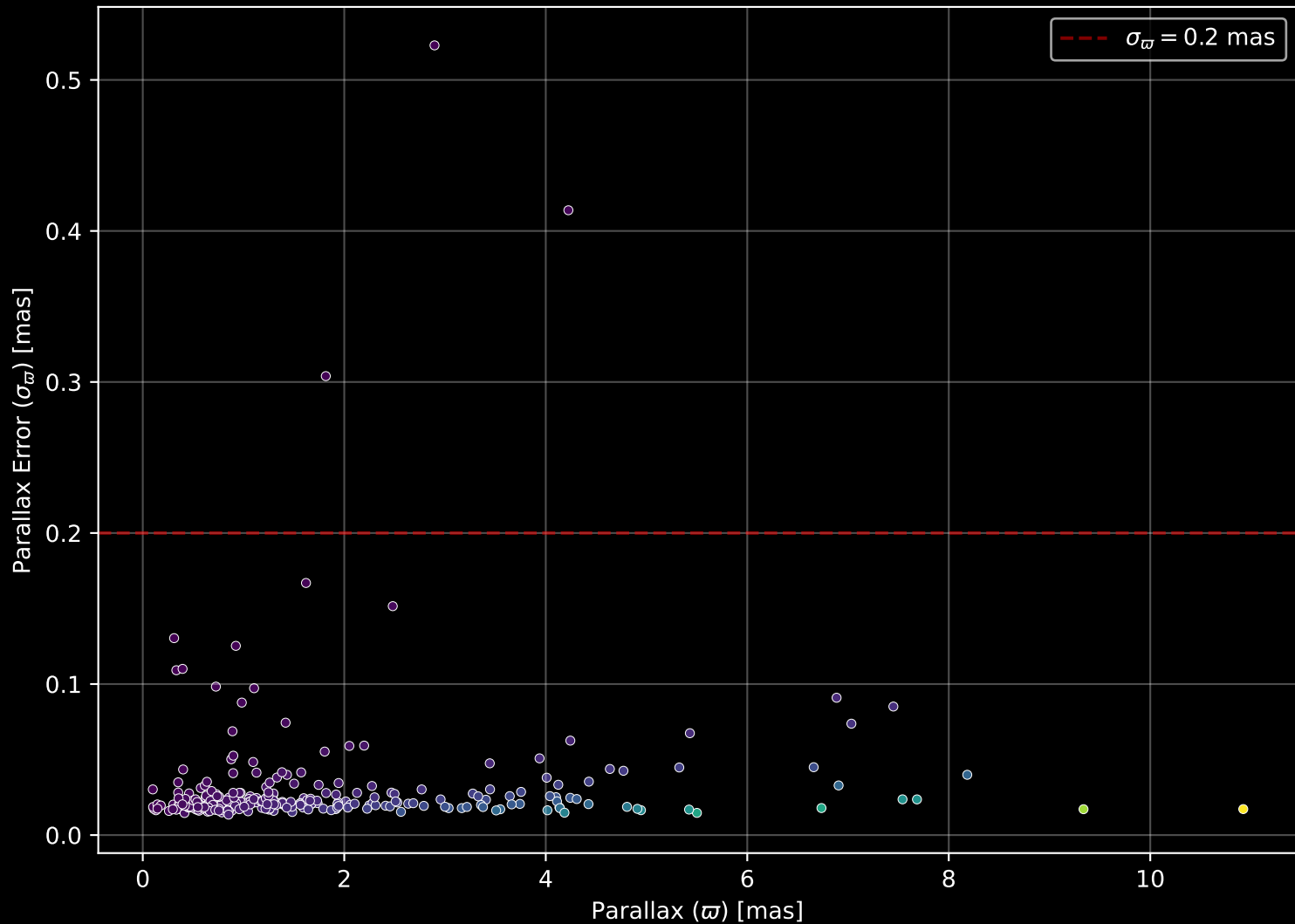
APOGEE DR17 Field: [K2_C11_001+07_btx] Parallax Quality (n= 286)
