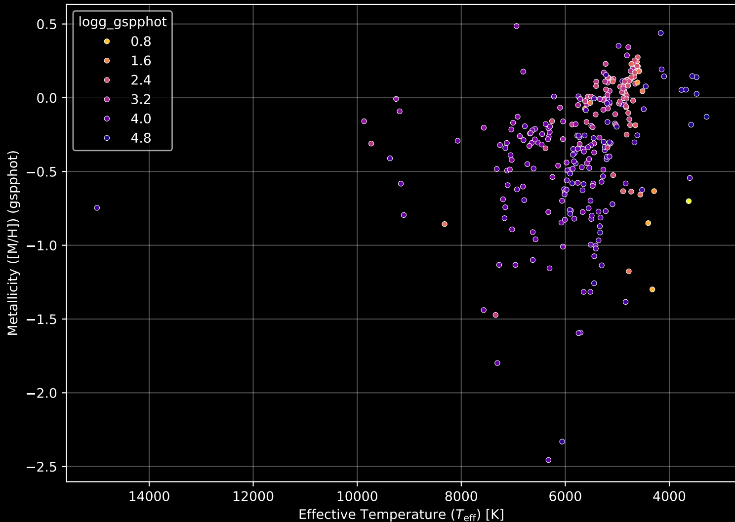
APOGEE DR17 Field: [K2_C11_001+07_btx] Stellar Population Parameters (n= 286)
