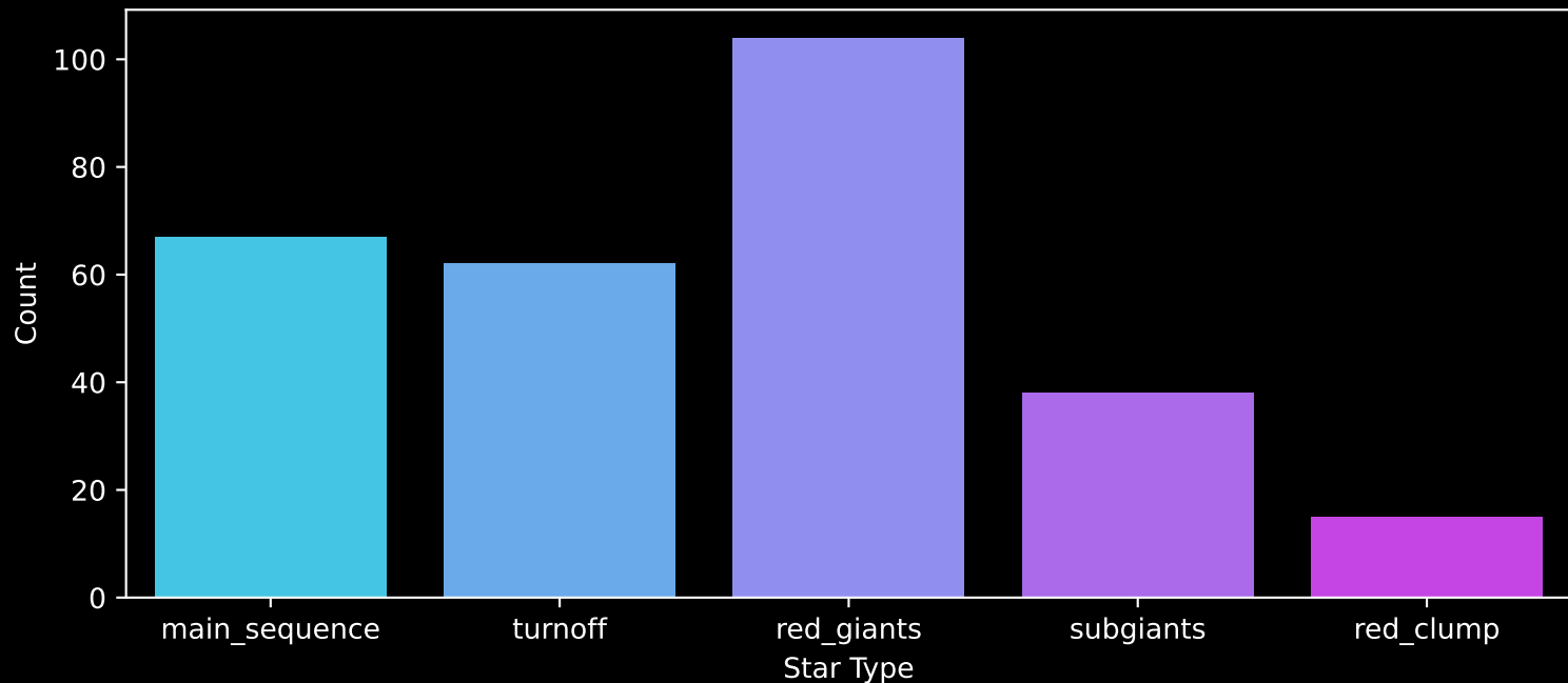
APOGEE DR17 Field: [K2_C11_001+07_btx] Count plot of Star Type
