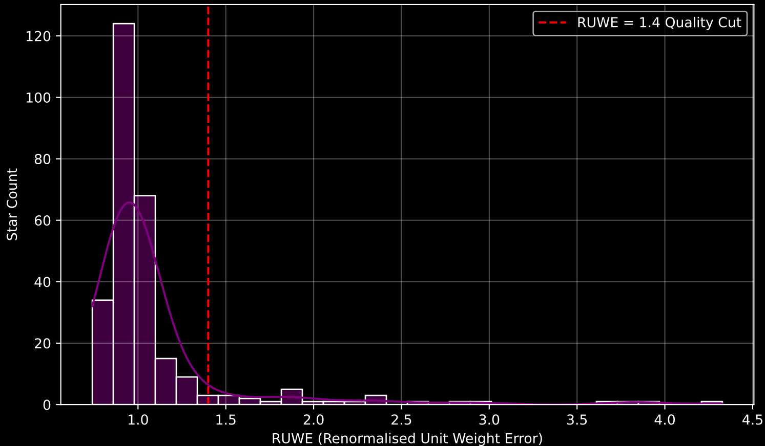
GAPOGEE DR17 Field [K2_C11_001+07_btx] RUWE Distribution (n= 277)
