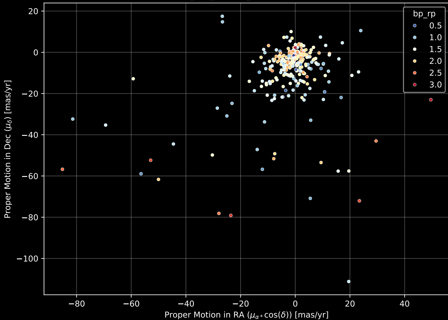
APOGEE DR17 Field: [K2_C11_001+07_btx] Proper Motion Diagram (n= 286)
